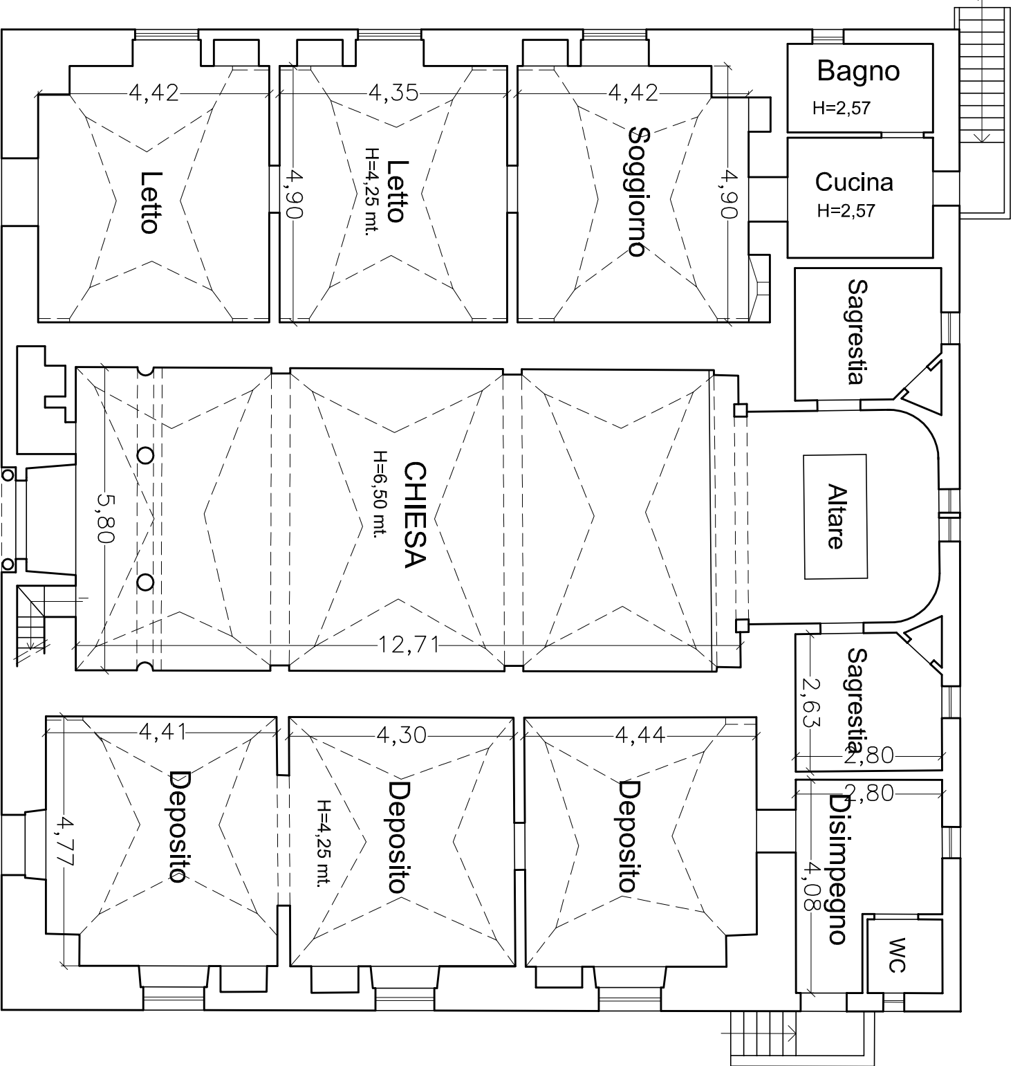
PIANO TERRA
