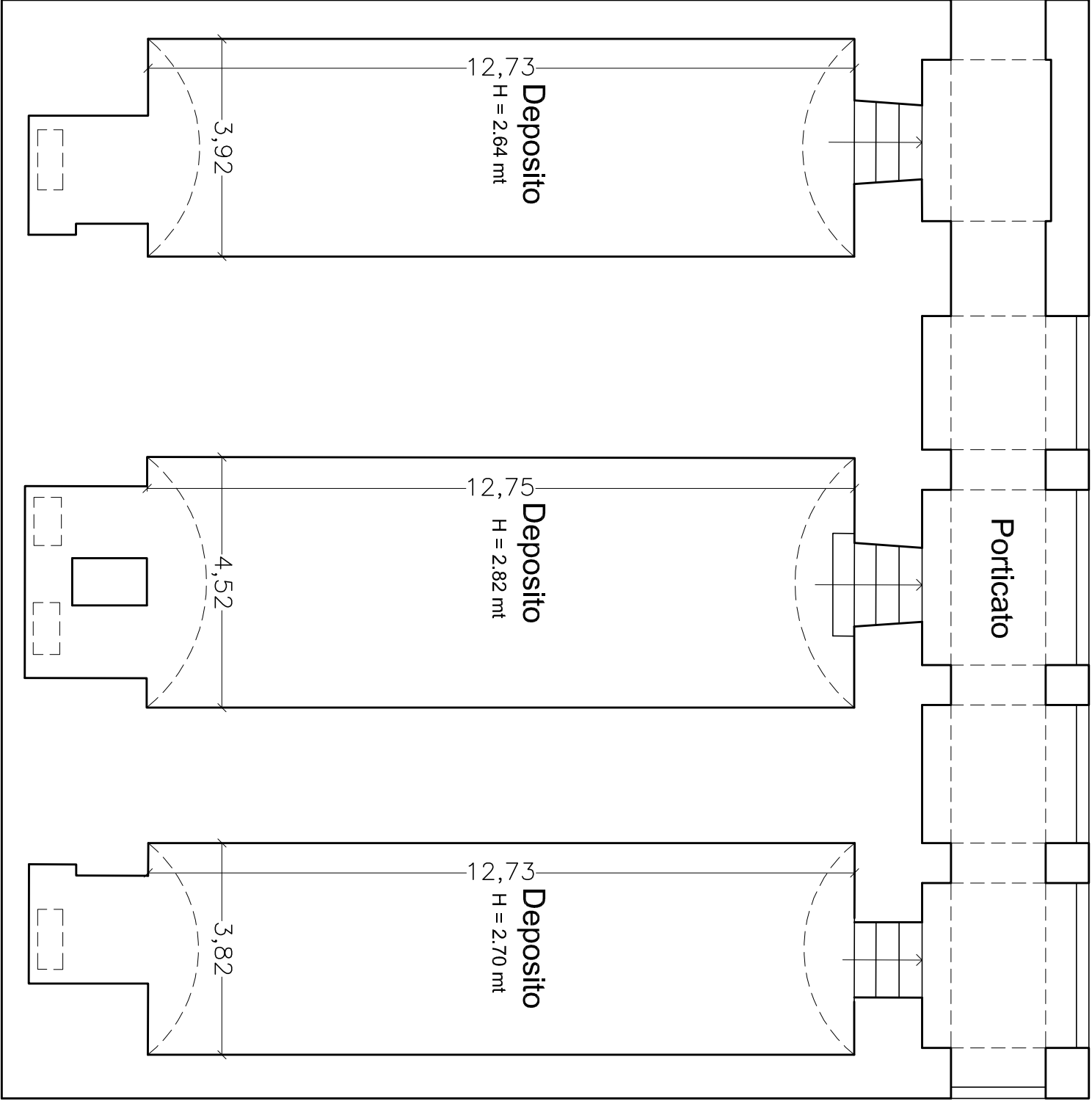
PIANO SEMINTERRATO
