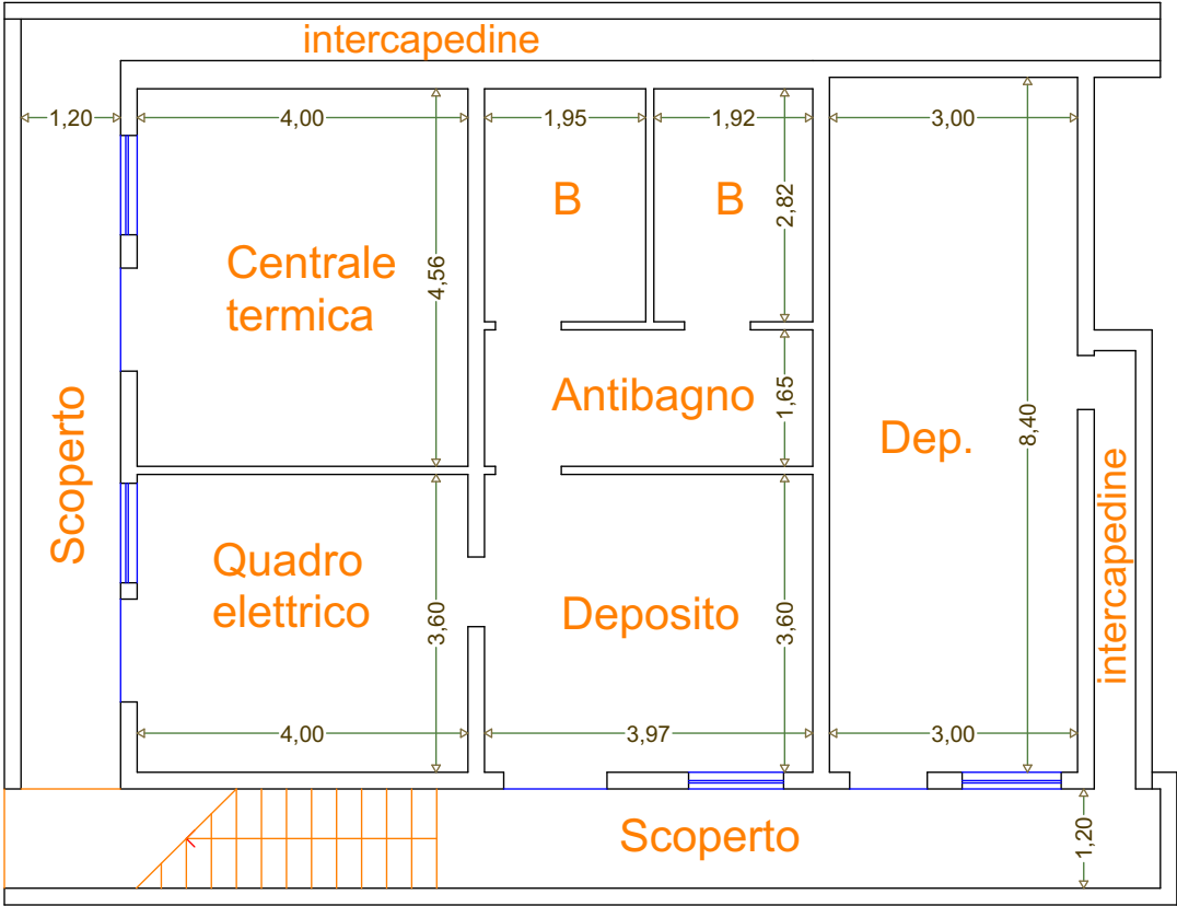
PIANO INTERRATO H = 2.40 mt
